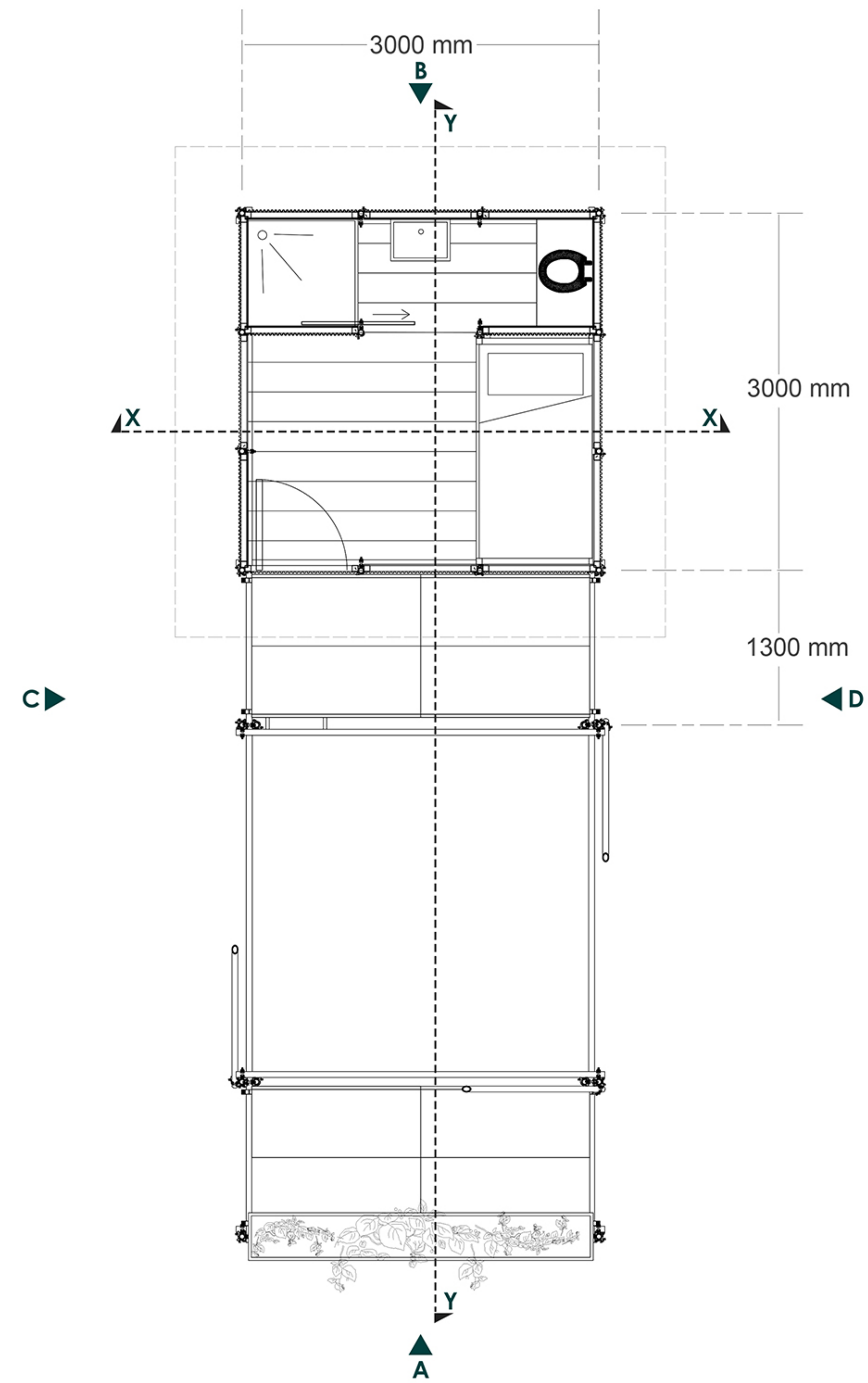
PLAN - SINGLE MODULE
